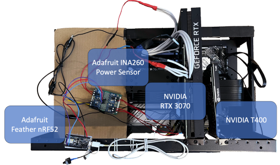
(b) Implementation of the block diagram
