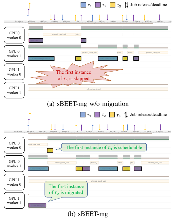
Figure 11: Job migration case study 1
