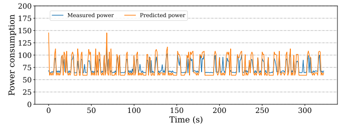
Figure 9: Trace of actual and predicted power consumption
