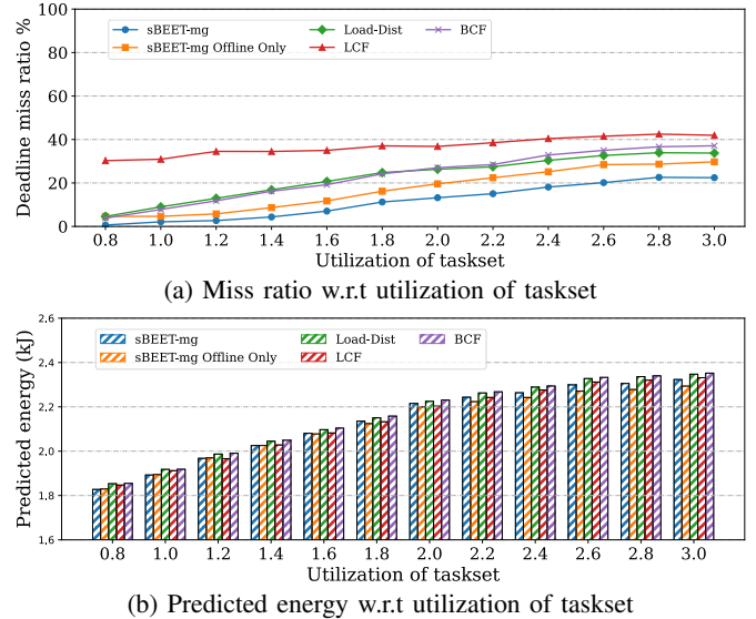
Figure 13: Simulation results of GPU configuration in Table IX
