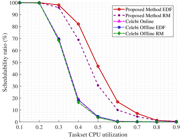
Fig. 7: Scheduler performance for different CPU utilization
